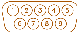
RC-500 Control head mounted view of 9 pin female connector
